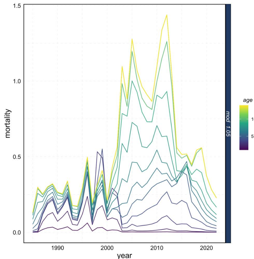
Figure 9. Estimates of Chilean hoki fishing mortality at age for model 1.04.
